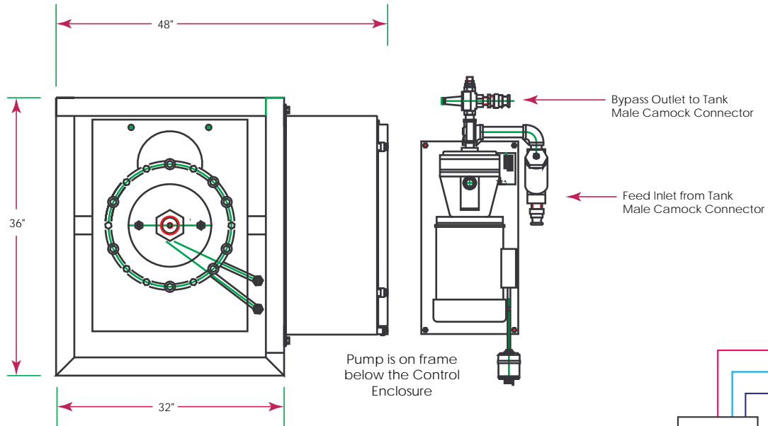
VSEP Series P-50 Footprint Drawing (Tank not Shown)
