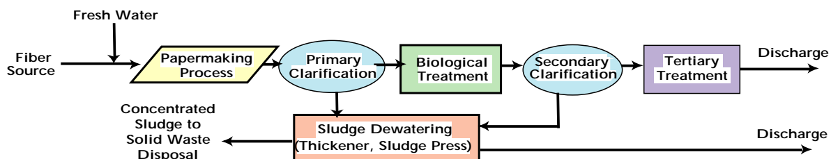
Figure 1 Conventional End of Pipe Effluent Treatment System
